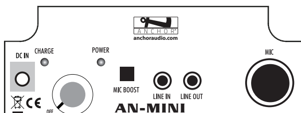
(AN-MINI Back Panel)
